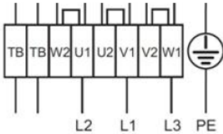
High speed \Delta -Connection
